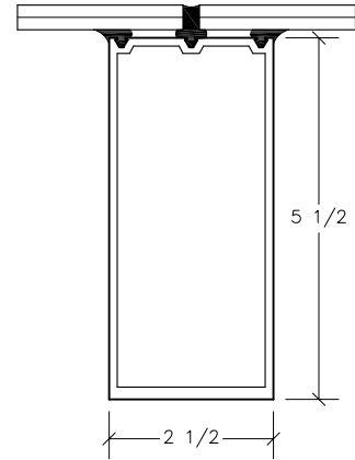
5 1/2" x 2 1/2" NOSELESS TRANSOM
