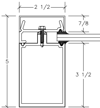
5" x 2 1/2" HEAD, JAMB AND SILL FRAME
