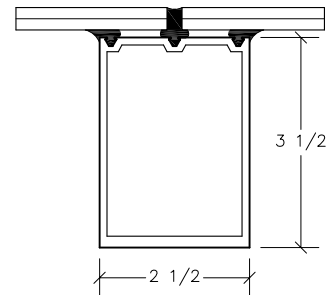
3 1/2" x 2 1/2" NOSELESS TRANSOM
